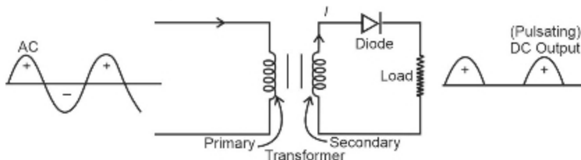
Figure: Half wave rectifier circuit diagram and waveform
