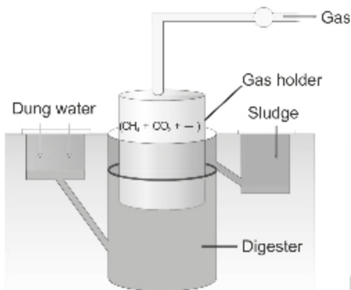
Fig : A typical biogas plant
