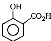
Salicyclic acid
