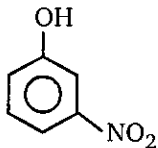
(m-nitrophenol)
