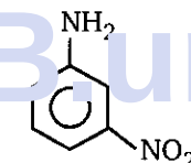
(m-nitro aniline)
