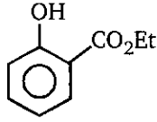
Ethyl salicylate
